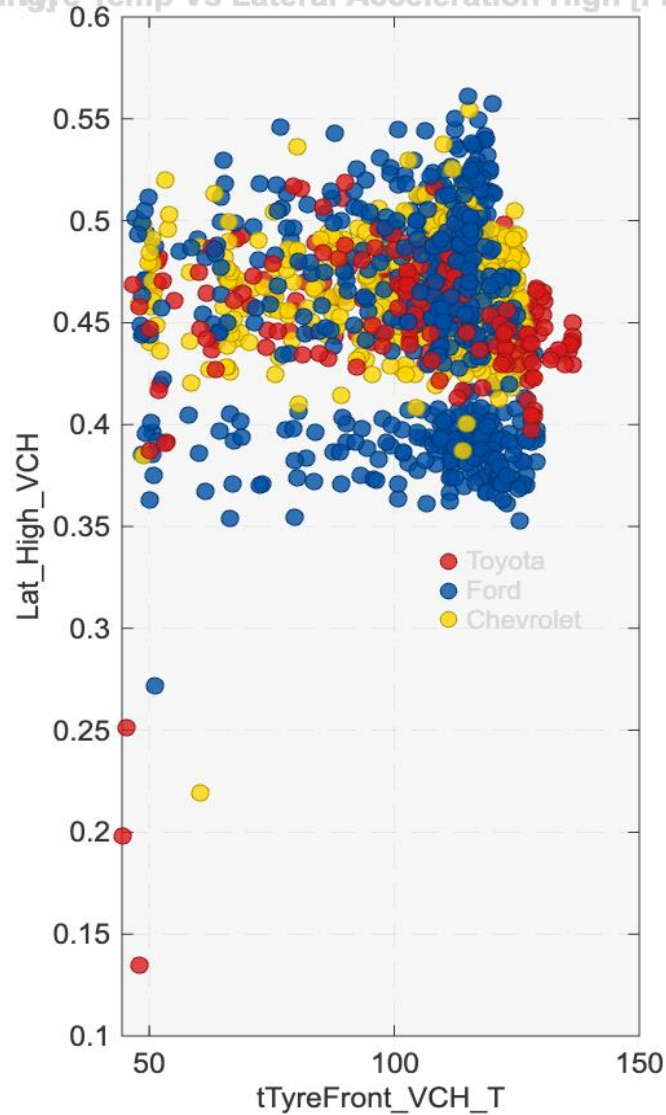
Tyre Temp Vs Lateral Acceleration High [Flying]
