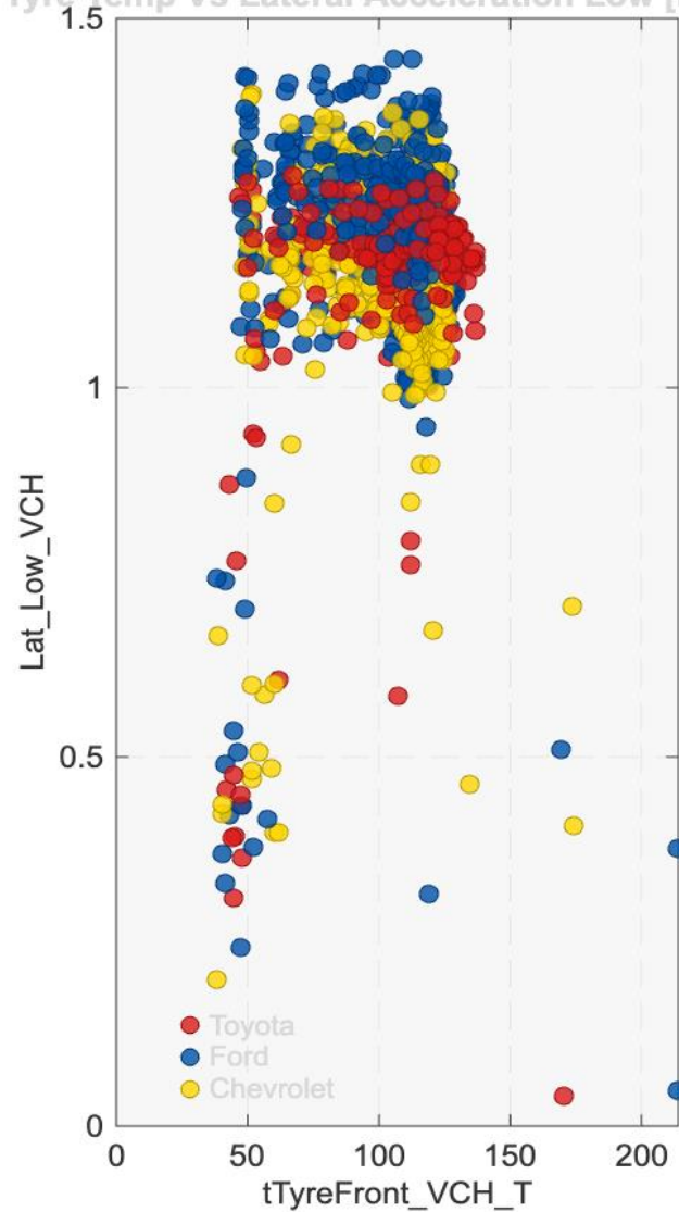
Tyre Temp Vs Lateral Acceleration Low [Flying]
