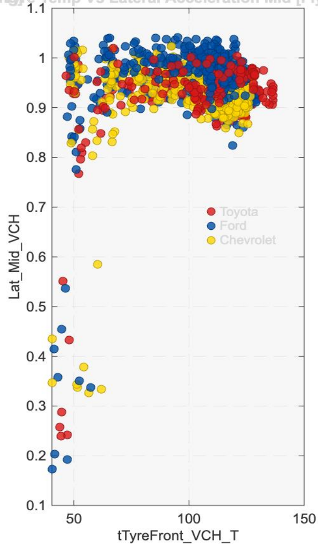
Tyre Temp Vs Lateral Acceleration Mid [Flying]
